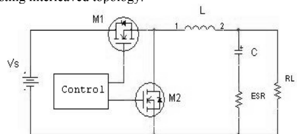
Fig.1 Synchronous rectifier buck converter
