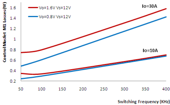
Fig. 2 Effect of switching frequency on Control MOSFET Losses
